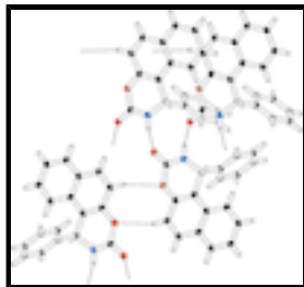
Fig. 2. The partial packing of (I), which shows that molecules are dimerized which are inter-linked in one dimensional infinite polymeric chains.
